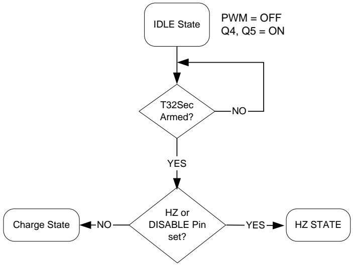
Figure 42. IDLE State
