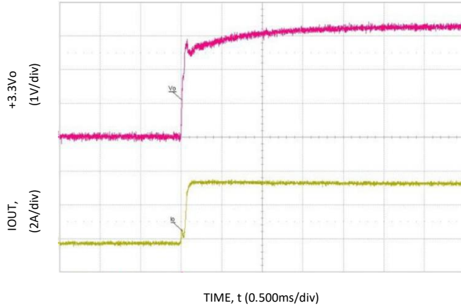
Fig 10: 3.3V Turn-On
