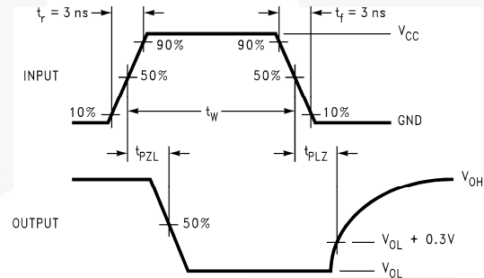
Figure 5. AC Waveforms
