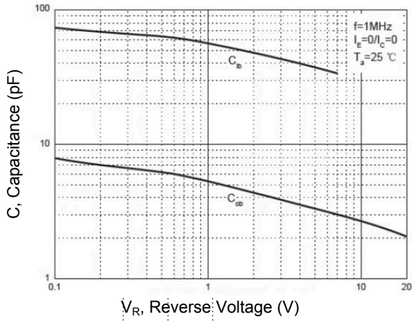
Figure 7. Capacitance Characteristics
