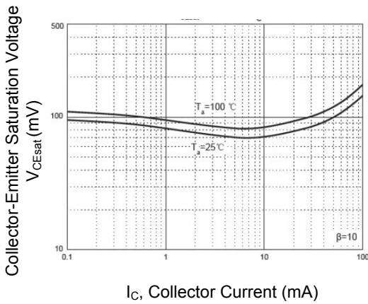
Figure 3. Collector-Emitter Saturation Voltage vs. Collector Current
