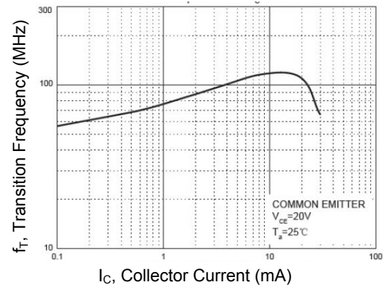
Figure 6. f_T vs. Collector Current
