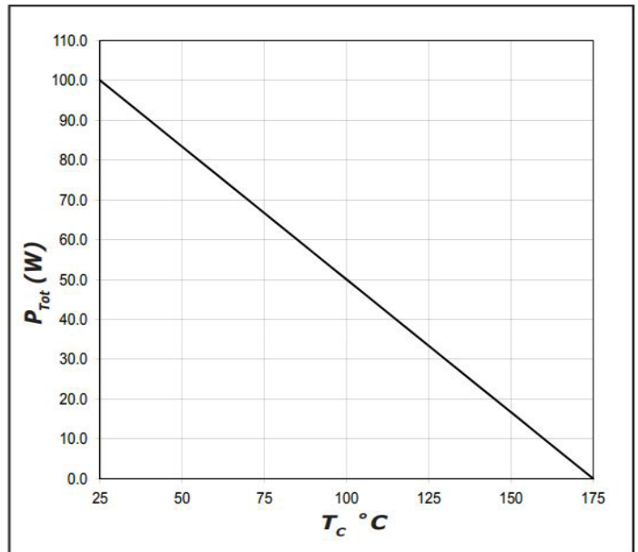
Figure 4 Power Derating
