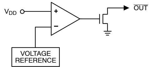
Figure 2. Block Diagram
