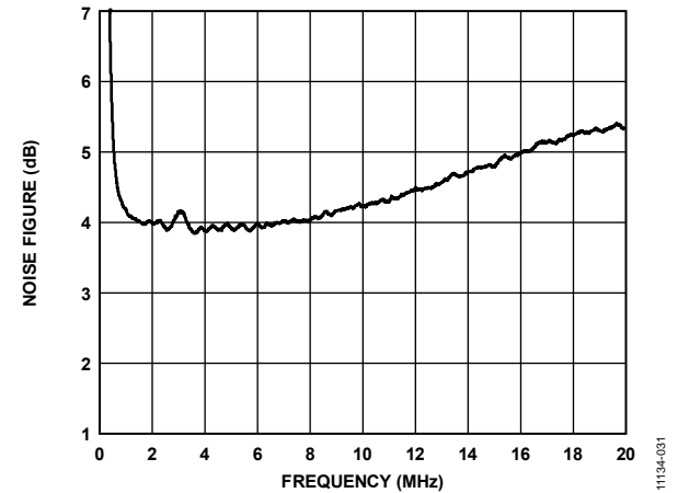
Figure 30. Noise Figure vs. Frequency R_S = R_{IN} = 100\Omega , LNA Gain = 17.9 dB, PGA Gain = 30 dB, V_{GAIN} = 1.6V
