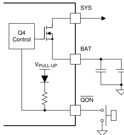
Figure 8-11. \overline{QON} Circuit
