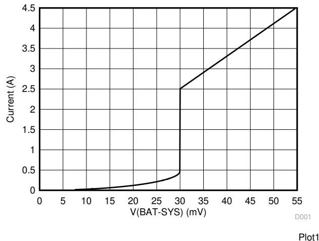
Figure 8-9. BAFET V-I Curve
