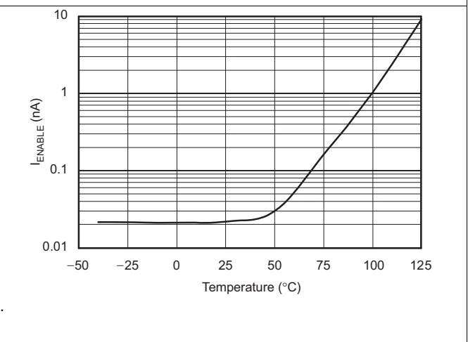
Figure 24. I_{ENABLE} vs Temperature
