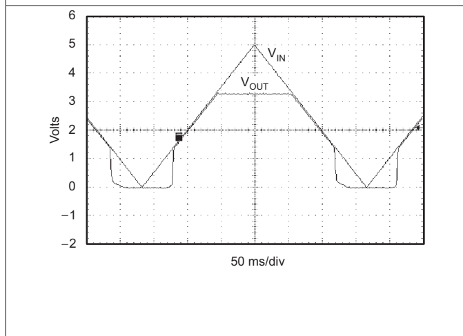
Figure 23. TPS73233 Power Up and Power Down
