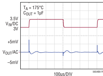
Figure 4. 175^{\circ}\text{C} Output Response to 0.5V Ripple on V_{\text{IN}}
