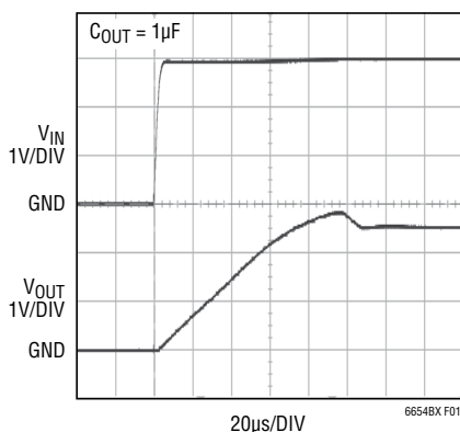
Figure 1. 25^{\circ}\text{C} Turn-On Characteristics of LT6654BX-2.5
