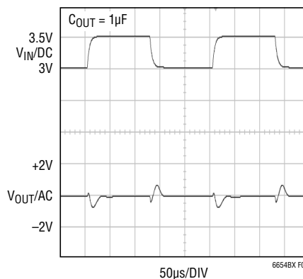
Figure 3. 25^{\circ}\text{C} Output Response to 0.5V Ripple on V_{\text{IN}}
