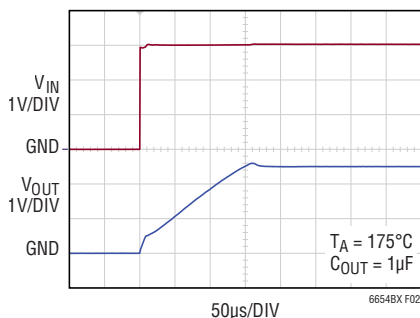
Figure 2. 175^{\circ}\text{C} Turn-On Characteristics of LT6654BX-2.5
