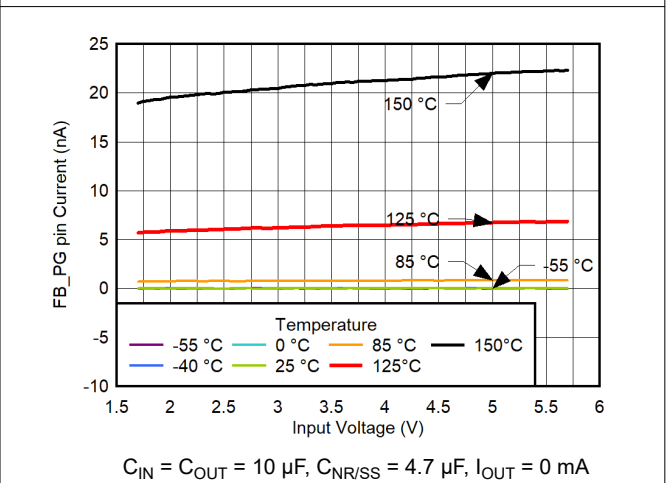
Figure 6-100. FB\_PG Pin Current vs V_{IN} and Temperature
