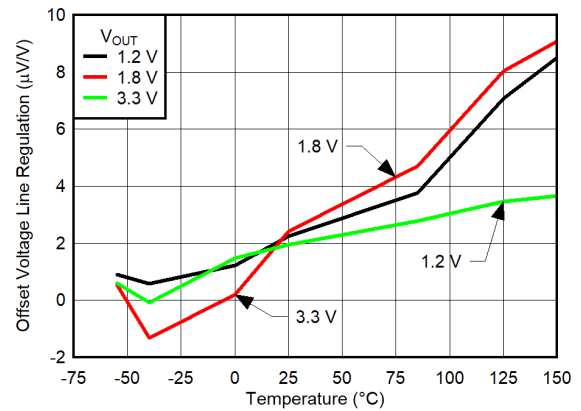
Figure 6-50. V_{OS} Line Regulation
