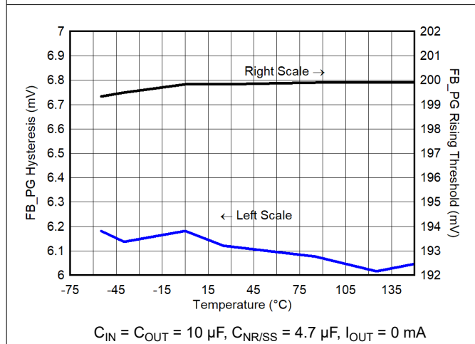
Figure 6-99. V_{FB\_PG} Hysteresis and Threshold vs Temperature
