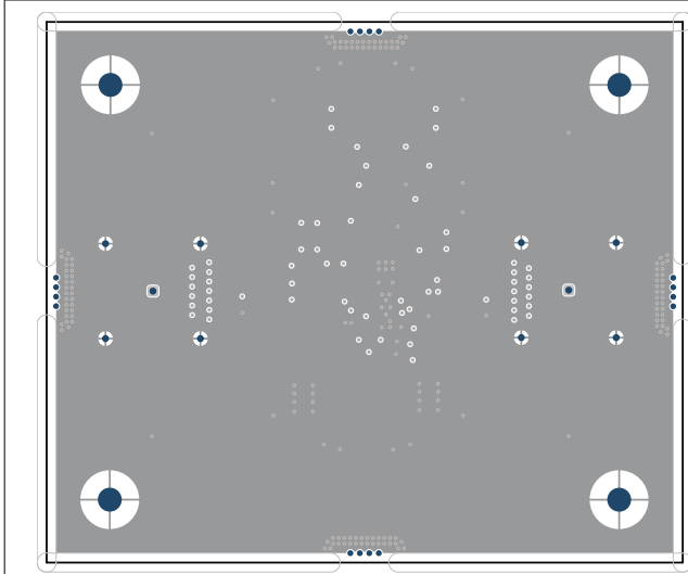
Figure 8-21. Mid Layer 1 Routing
