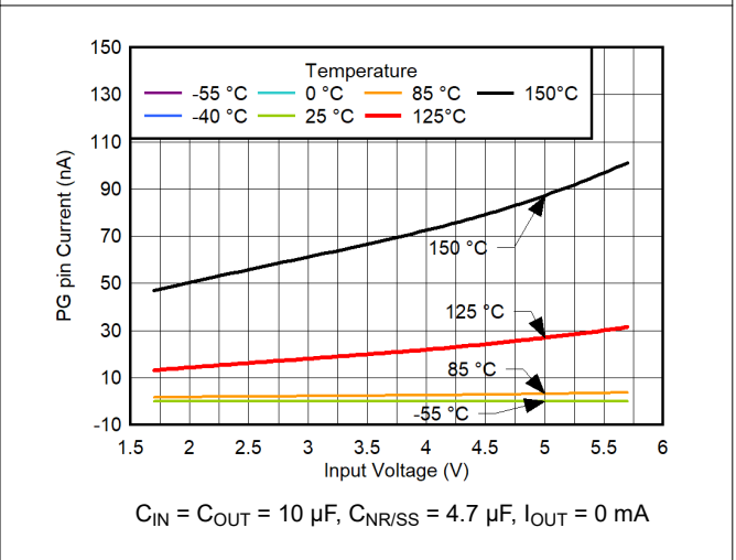
Figure 6-102. PG Pin Current vs V_{IN} and Temperature
