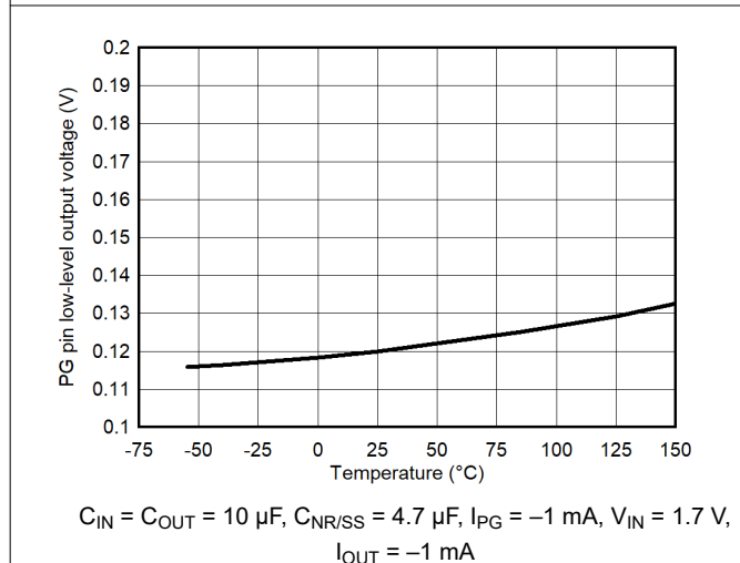
Figure 6-101. V_{PG} Low-Level Output Voltage vs Temperature
