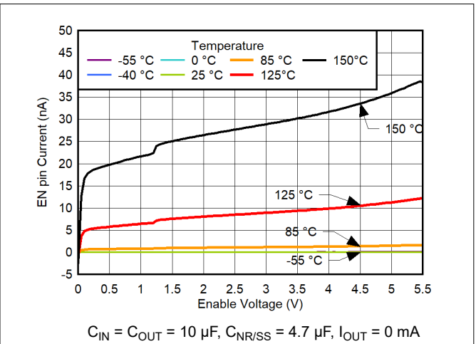
Figure 6-98. EN Pin Current vs Enable Voltage and Temperature for V_{IN} = 5.7\text{ V}
