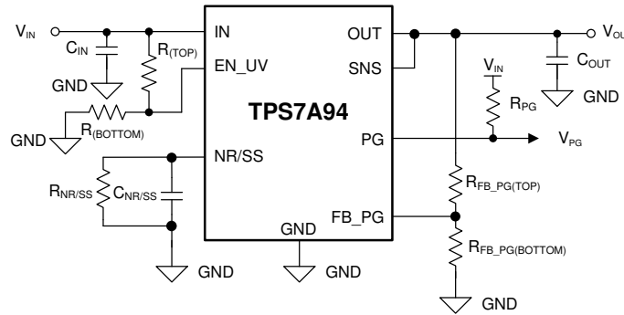
Figure 8-16. Typical Circuit
