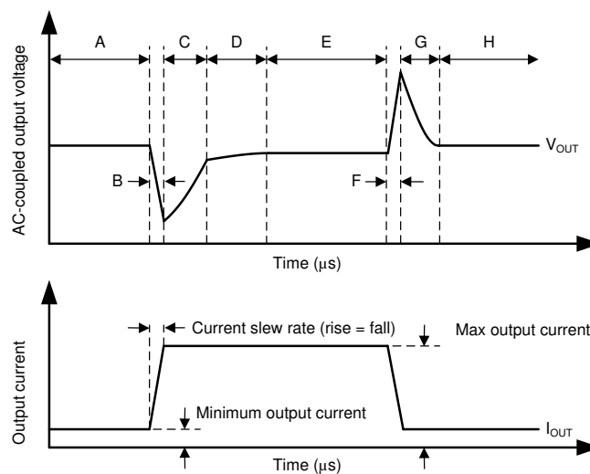
Figure 8-18. Load Transient Waveform
