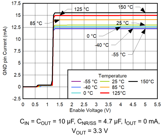
Figure 6-79. GND Pin Current vs V_{EN} and Temperature for V_{IN} = 1.7\text{ V} (Dropout Operation)
