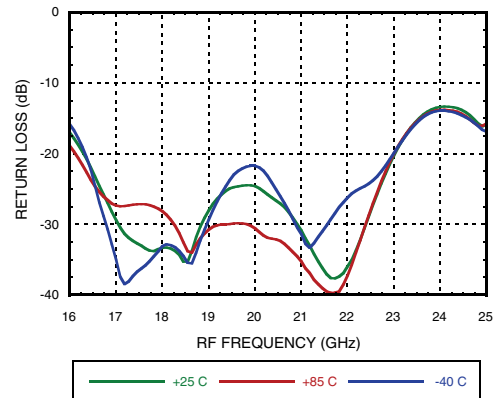
RF Return Loss vs. Temperature
